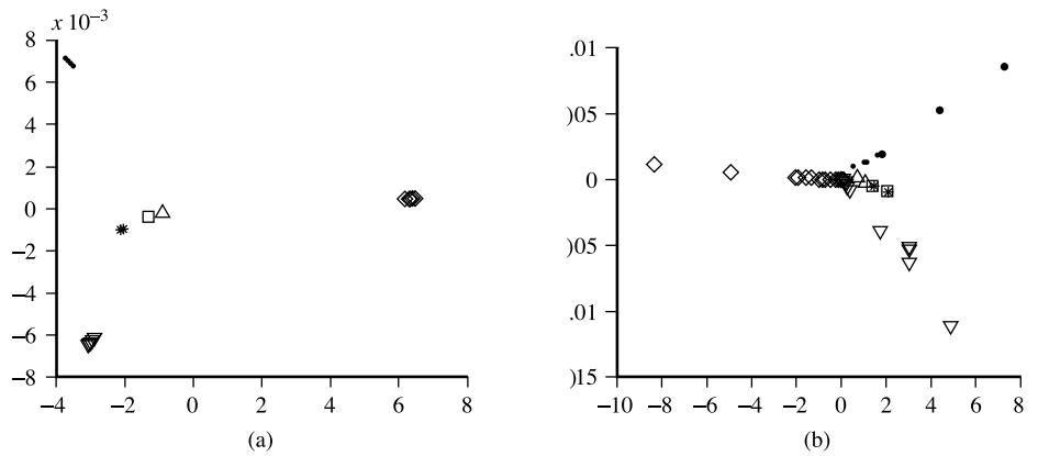
Figure 10.11 2-D embedding of the WWW images. (a) The image graph is constructed using block-level link analysis. Each color (shape) represents a semantic category. Clearly, they are well separated. (b) The image graph was constructed based on traditional perspective that the hyperlinks are considered from pages to pages. The image graph was induced from the page-to-page and page-to-image relationships.
